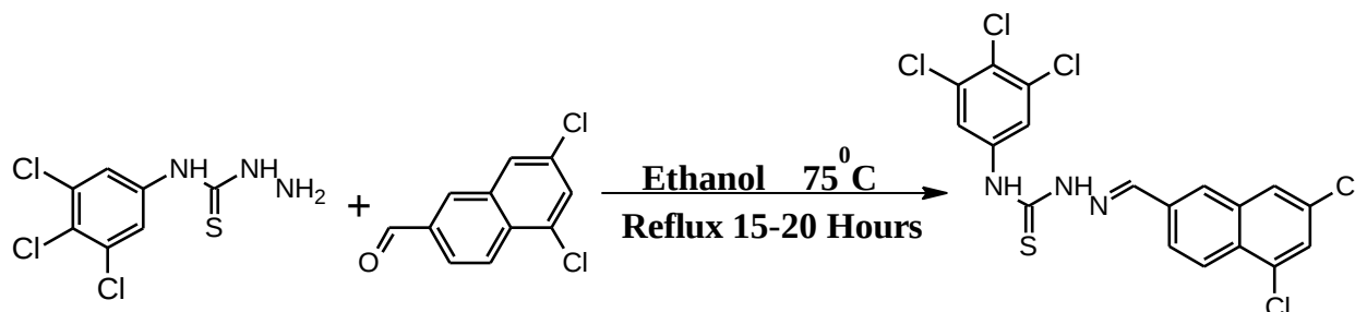
Scheme 1. Scheme for synthesis of (2E)-2-[(5,7-dichloronaphthalen-2-yl)methylidene]-N-(3,4,5-trichlorophenyl)hydrazine-1-carbothioamide
