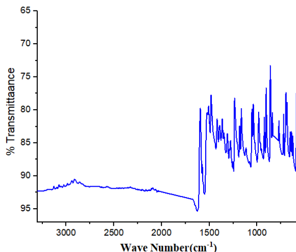
Figure 1: FTIR of Structure of (2E)-2-[(5,7-dichloronaphthalen-2-yl)methylidene]-N-(3,4,5-trichlorophenyl)hydrazine-1-carbothioamide
