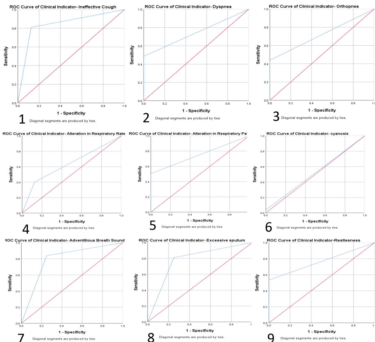
Figure 6: AUROC of clinical indicators
