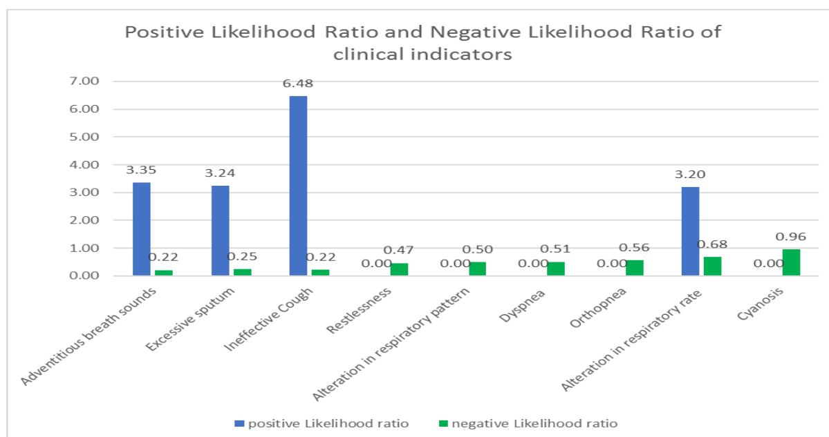
Figure 4. Likelihood Ratio
