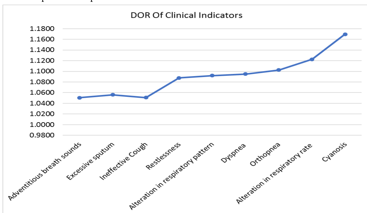
Figure 5. Diagnostic odds ratio
