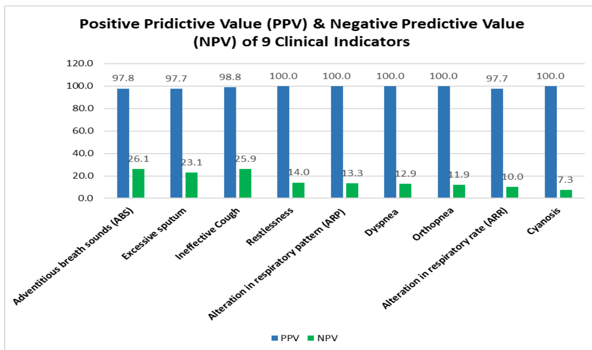
Figure 3. PPV & NPV
