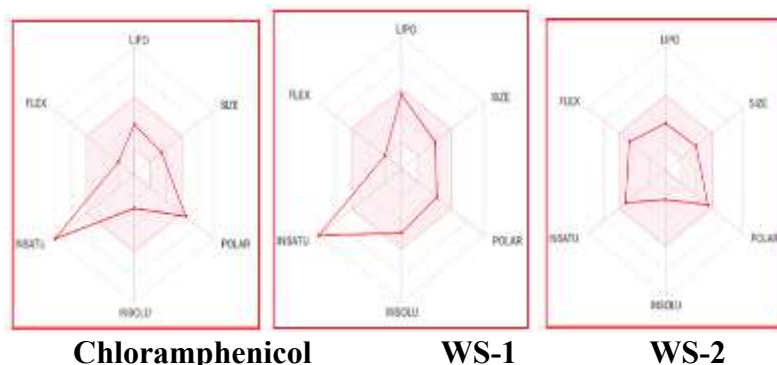
Figure 13: Bioavailability radar
