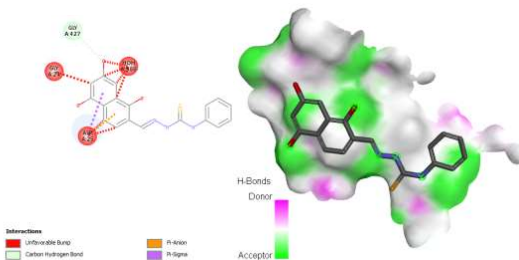
Figure Interaction (a) and binding pattern (b) of WS-2 with Alpha-glucosidase protein as a receptor.
