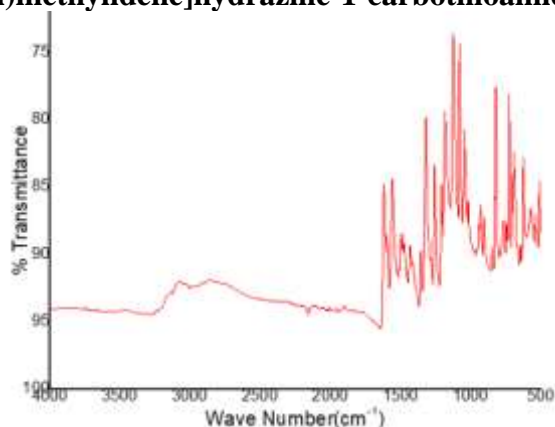
Figure 2: FTIR of Structure of (2E)-N-phenyl-2-[(1,5,7-trihydroxynaphthalen-2-yl)methylidene]hydrazine-1-carbothioamide
