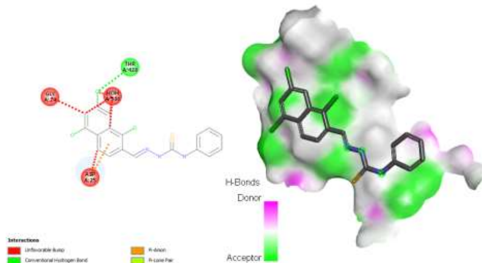
Figure Interaction (a) and binding pattern (b) of WS-1 with Alpha-glucosidase protein as a receptor.
