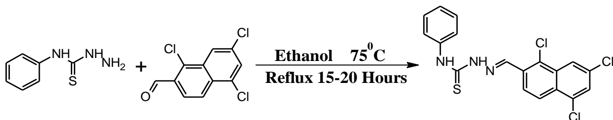
Scheme 1. Scheme for synthesis of (2E)-N-phenyl-2-[(1,5,7-trichloronaphthalen-2-yl)methylidene]hydrazine-1-carbothioamide
