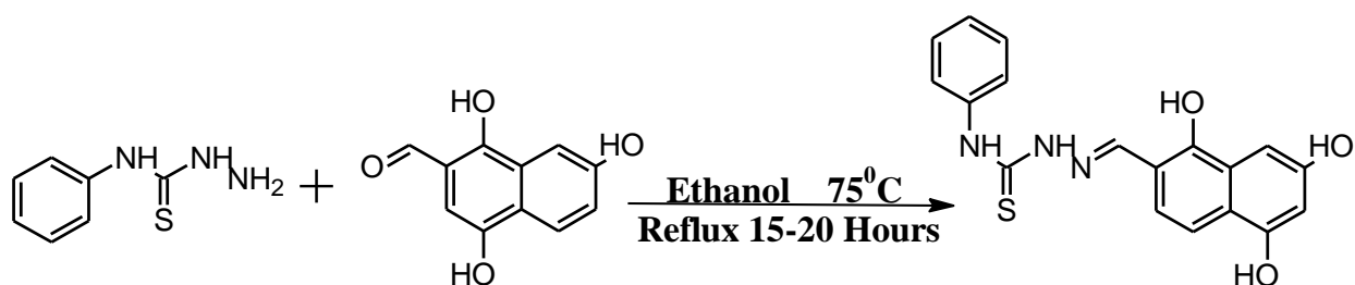
Scheme 2. Scheme for synthesis of (2E)-N-phenyl-2-[(1,5,7-trihydroxynaphthalen-2-yl)methylidene]hydrazine-1-carbothioamide
