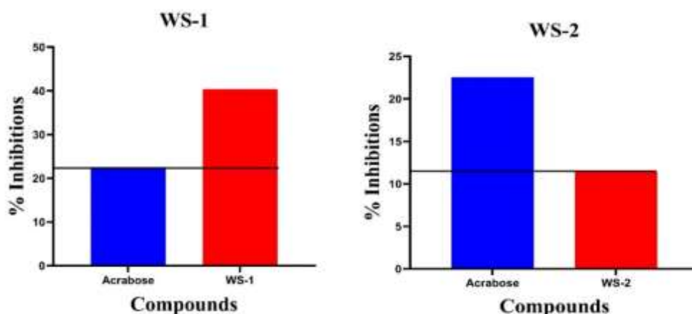
Figure 2: Graphical presentation of alpha glucosidase inhibition of WS-1 and WS-2 in comparison to Acarbose as reference Computational Study
