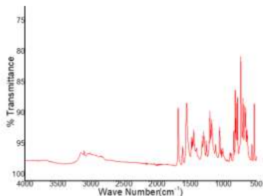
Figure 1: FTIR of Structure of (2E)-N-phenyl-2-[(1,5,7-trichloronaphthalen-2-yl)methylidene]hydrazine-1-carbothioamide
